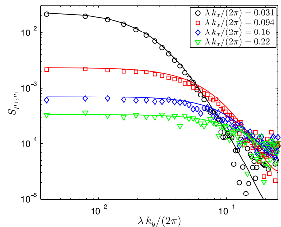
FIG. 1 (color online). Discrete structure factor S_{\rho_1, v_{\parallel}^{(1)}} from quasi-two-dimensional DSMC runs with L_x = 64\lambda , L_y \perp 512\lambda , and L_z = 2\lambda , for several wave numbers k_x = \kappa_x \times 2\pi/L_x (see legend), compared to the discrete equivalent of the continuum prediction (4) (solid lines of the same color). Note that for a fixed k_x we expect the structure factor to decay as k_y^{-4} .
