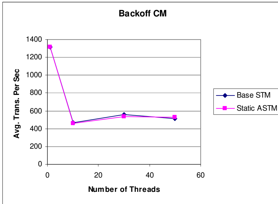
Figure 9 - Backoff CM
