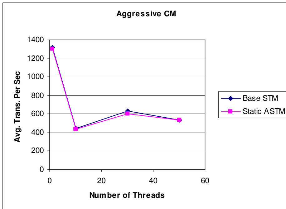
Figure 10 - Aggressive CM
