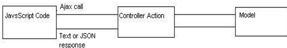
Figure 3: The Application Flow
