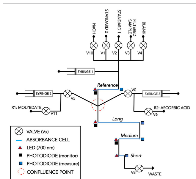
FIGURE 2 | Schematic flow diagram of Sensor 2. This sensor is the latest version designed and manufactured at the National Oceanography Centre Southampton. Absorbance cells: Long: 98 mm; Medium: 35 mm; Short: 2.5 mm. The reference cell (35 mm, but not used in this work) may be used to determine the absorbance of the sample prior to addition of the reagents.
