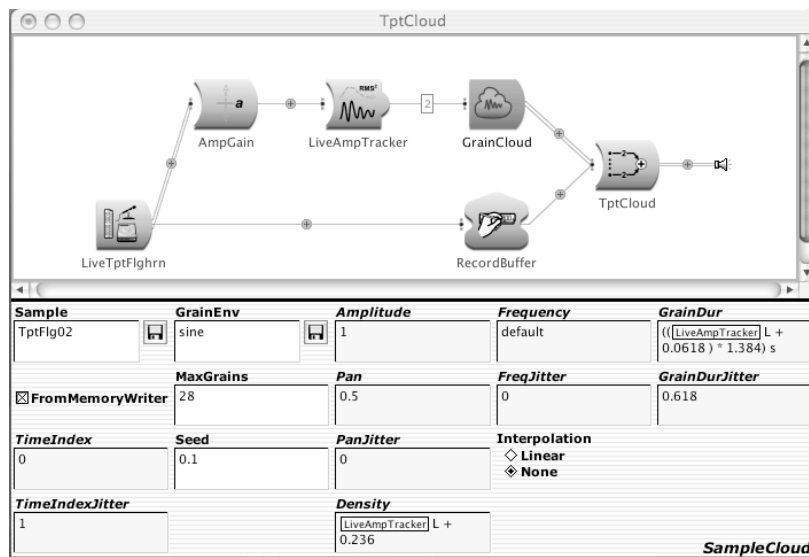
Figure 4. Kyma graphic structure for the TptCloud algorithm, showing detailed parameters, including random and trumpet/flugelhorn amplitude functions (via ‘LiveAmpTracker’), for the SampleCloud (‘GrainCloud’) Sound.
