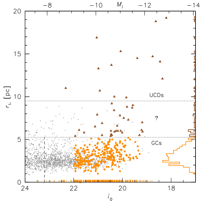
Figure 3. Half-light radius vs. i -band magnitude for compact stellar systems. Small gray points show GC candidates in the central HST /ACS field (Jordán et al. 2009), while larger symbols show objects in the spectroscopic sample. Dotted lines show our diagnostic boundaries for GCs, UCDs, and uncertain/transition objects, with accordingly different symbols for the spectroscopic objects in these regions. Spectroscopically confirmed objects with no size measurements are plotted as tick marks near r_h = 0 . The vertical dashed line shows the approximate globular cluster luminosity function (GCLF) turnover magnitude. A histogram on the right-hand side shows the number of objects in size bins. There are another 20 UCDs with r_h > 20 pc that are not visible on this plot.
