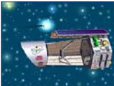
Kepler Mission
