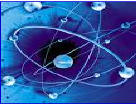
Quantum Mechanics
