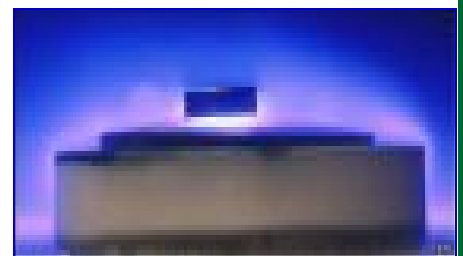
Superconductivity
