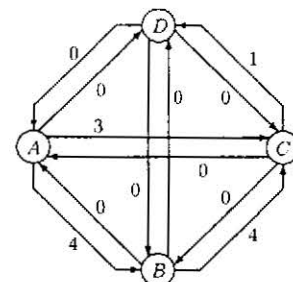
Figure 1: Directed graph G .
