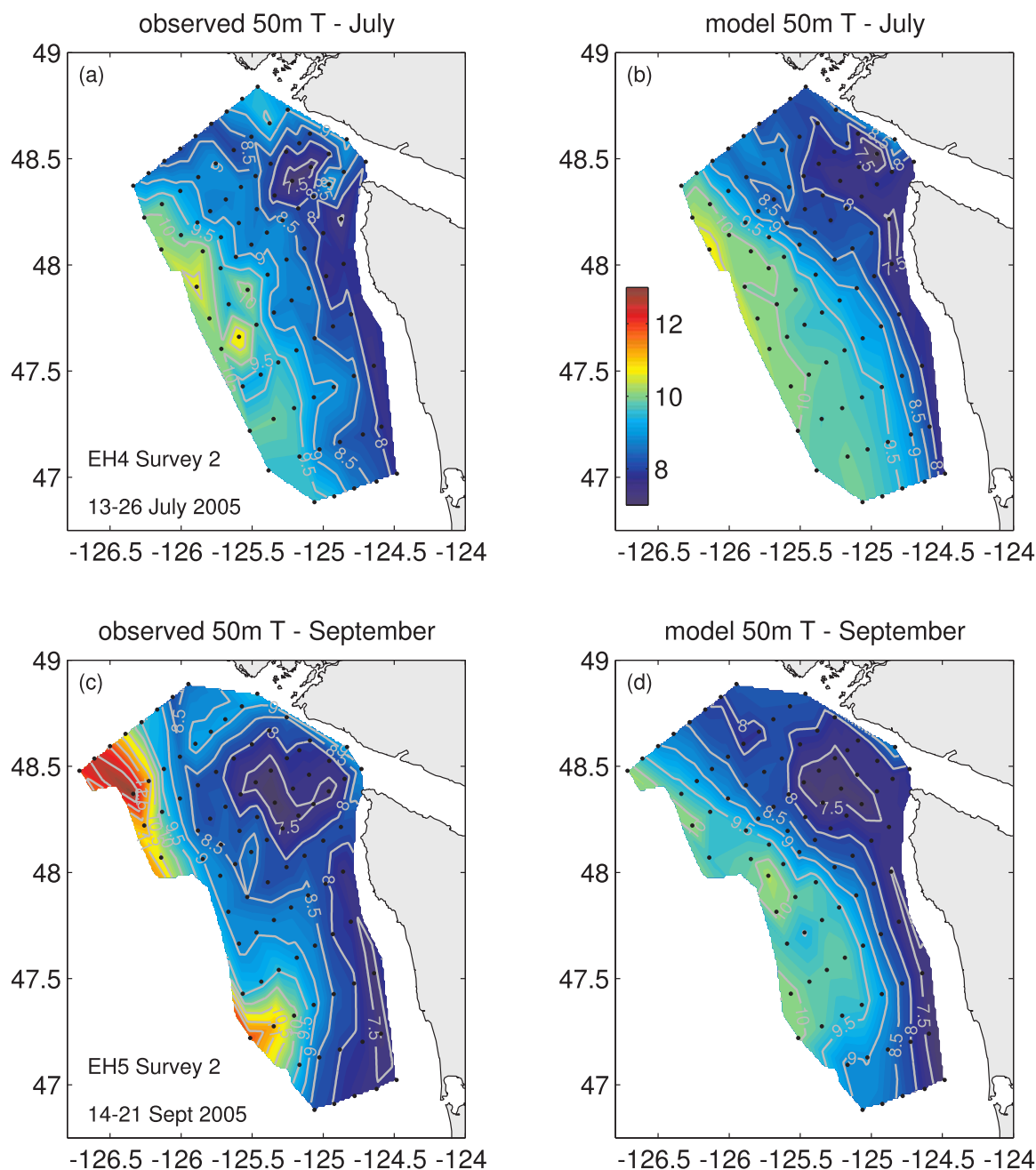
Figure 6. Maps of modeled and observed temperature at 50 m during (a and b) July and (c and d) September 2005. Model output is subsampled to the same locations and times as the observations.
