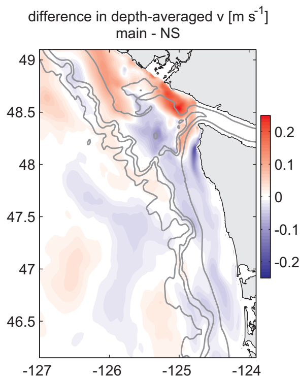
Figure 12. Difference in depth-averaged along-shelf velocity, v , between the main run and no strait (NS) run, averaged over the period June-September. Red and blue indicate stronger poleward and equatorward velocity, respectively, in the main run. The along-shelf direction is defined by the radial coordinate system described in section 2.2.
