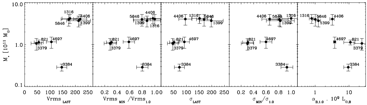
Figure 18. Correlation between total stellar mass and V_{\text{rms}} , V_{\text{rms}}/V_{\text{rms},1.0} , \sigma_{\text{LAST}} , \sigma_{\text{MIN}}/\sigma_{1.0} and the \alpha parameter.
