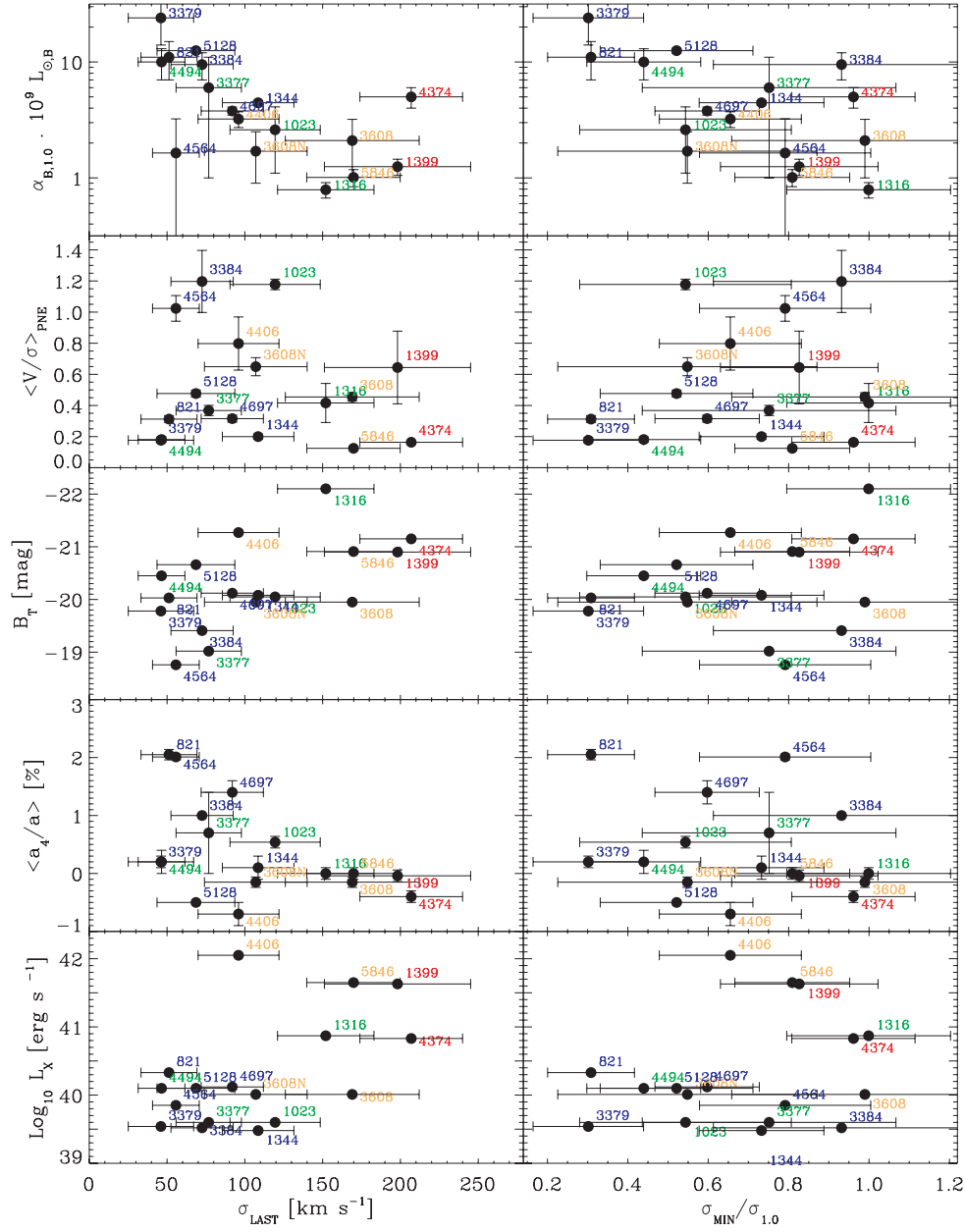
Figure 17. Same as Fig. 16, but for \sigma_{\text{LAST}} (left-hand panels) and \sigma_{\text{MIN}}/\sigma_{1.0} (right-hand panels).
