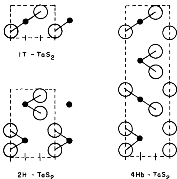
FIG. 1. Crystal structures shown along the (11\bar{2}) plane of three phases of \text{TaS}_2 . Note the similarity of the van der Waals gap symmetry in 2H- \text{TaS}_2 and 4Hb- \text{TaS}_2 .
