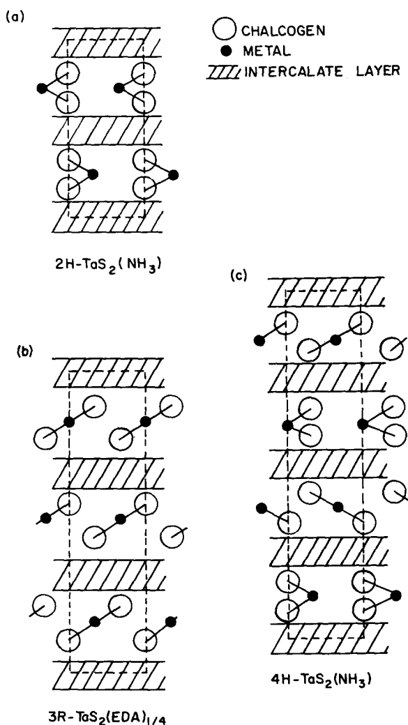
FIG. 4. Crystal structures for intercalated compounds shown along the (11\bar{2}0) plane (compare Fig. 1) deduced from intensity distributions of (10l) and (11l) lines for (a) 2H-TaS 2 (NH 3 ) and 2H-NbSe 2 (NH 3 ), (b) 3R-TaS 2 (EDA) 1/4 (intercalated 1T-TaS 2 ), and (c) 4H-TaS 2 (NH 3 ). Note the similarity of the van der Waals gap in (a) and (c).
