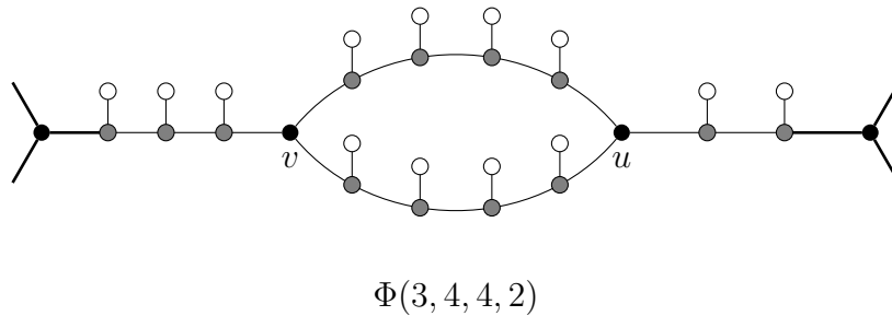
Figure 10: The configuration \Phi(t, a_1, a_2, s) .
