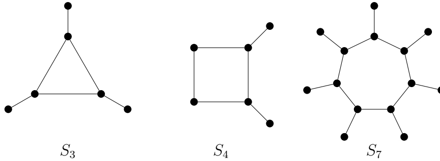
Figure 4: Exceptions in Theorem 8.
