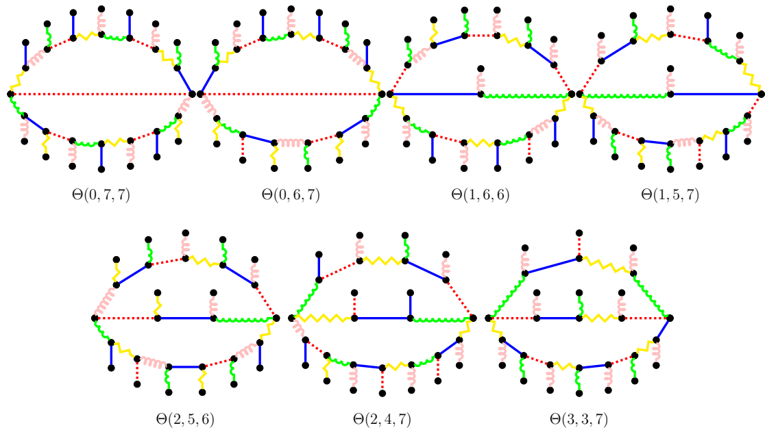
Figure 11: Strong edge-colorings of \Theta(t_1, t_2, t_3) . Style of line corresponds to color to make colors visible on a black and white print.
