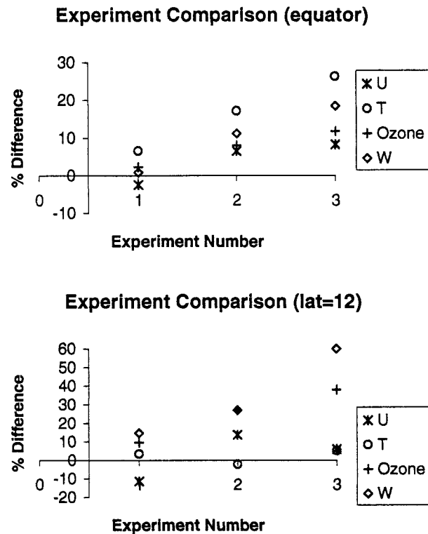
FIG. 16. Comparison between the amplitudes at the equator and 12^\circ latitude for the QBO variations in zonal wind, temperature, ozone volume mixing ratio, and vertical motion; these fields are calculated as a percent difference from the reference simulation. Percent difference for expt 1 calculated as 100(X_{\text{Expt}} - X_{\text{ref}})(X_{\text{ref}})^{-1} .
