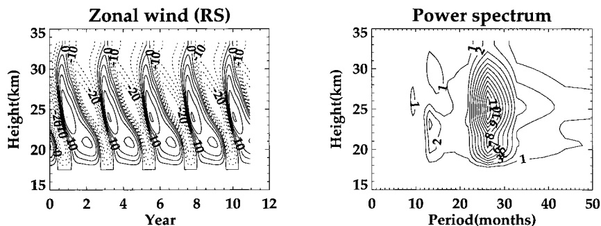
FIG. 3. (a) Time–height cross section of the zonal wind at the equator for the RS. Contour interval is 5 \text{ m s}^{-1} , and dotted contours represent easterly winds. (b) Amplitude of the modeled zonal wind power spectra over the equator for the reference simulation. Contour interval is 1 \text{ m s}^{-1} .
