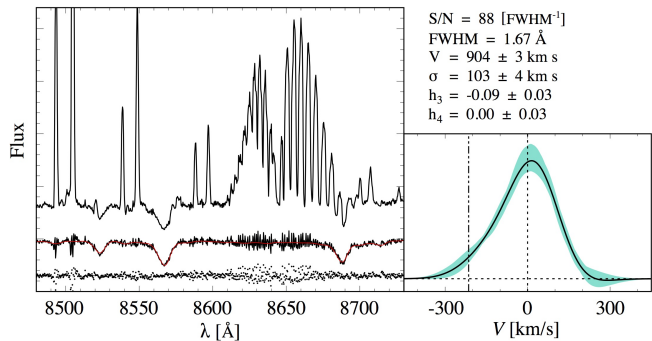
FIG. 6.— An example of an extracted stellar spectrum 1.5 arcmin from center of the galaxy NGC 3115. Left: A fiducial raw spectrum with galaxy stellar light and night-sky background (top); sky subtracted spectrum with best fit model overlaid in red (middle); and fitting residuals (bottom). Right: Best fitting parameterized LOSVD (solid black line). The envelope (solid cyan) shows the range of possible solutions as determined from 100 Monte Carlo realizations of the best fit model with added noise. The velocity axis has been shifted to the mean velocity of the measurement, and the vertical dot-dashed line marks the systemic velocity of the galaxy.
