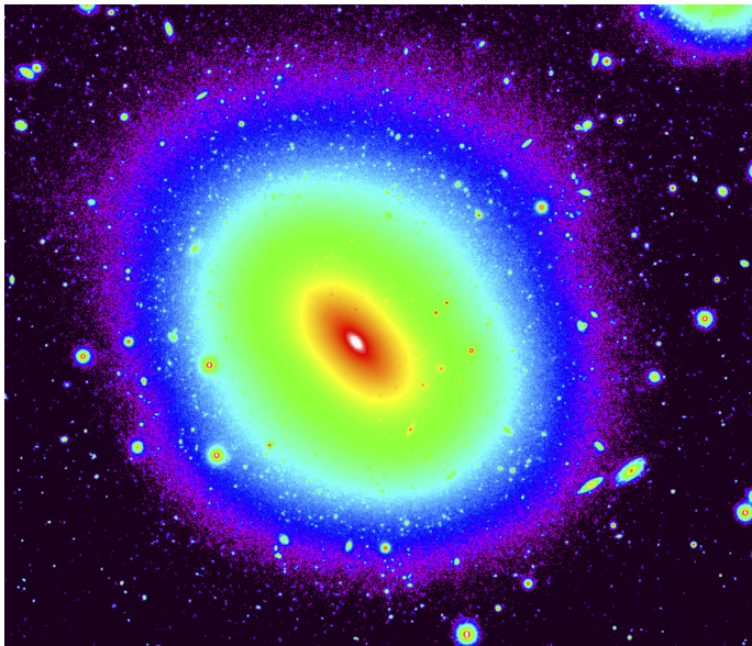
FIG. 13.— Two-dimensional photometry of NGC 3377. Left : g -band Subaru/Suprime-Cam image ( \sim 30 kpc field of view), with an arbitrary color scale used for contrast. Right : The top two panels show profiles of the isophote ellipticity and shape parameter (fourth-order cosine term a_4 > 0 is disk, < 0 is boxy, taken from literature studies in various optical filters; Jedrzejewski 1987; Michard & Simien 1988; Scorza & Bender 1995; Peletier et al. 1990; Goudfrooij et al. 1994). Both expressions of the data suggest a disk component embedded in a round and boxy bulge, which may be compared to the 1D rotation profile (bottom right panel) and to the 2D velocity map in Figure A1.
