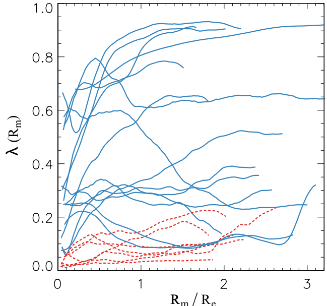
FIG. 10.— Radial profiles of the local stellar specific angular momentum proxy \lambda , for our sample galaxies. Blue solid curves denote centrally fast rotators and red dashed curves denote centrally slow rotators. A diversity of rotation profiles is seen beyond 1 R_e , with centrally slow rotators remaining relatively slow, and centrally fast rotators ranging from decreasing to constant to increasing \lambda .
