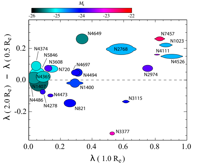
FIG. 11.— The radial gradient of specific stellar angular momentum, parameterized as the change in local \lambda between 0.5 and 2.0 R_e scales, vs. \lambda at 1.0 R_e . Each point is sized according to galaxy R_e (in physical units), while the shape and color reflect isophote flattening at 1 R_e and K -band absolute magnitude (see color bar at top), respectively. A fiducial division between fast and slow rotators is shown as a red vertical dashed line. There appears to be a pattern for lenticulars to have \Delta\lambda > 0 (radially increasing profiles) and fast-rotator ellipticals to have \Delta\lambda < 0 (radially decreasing).
