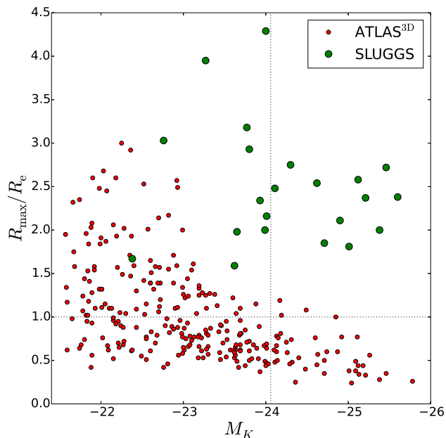
FIG. 1.— Radial extent of stellar-spectroscopy data, in units of the effective radius ( R_e ), versus galaxy K -band absolute magnitude. Horizontal and vertical dotted lines mark 1 R_e and the characteristic luminosity (Bell et al. 2003), respectively. A given instrument with a fixed field-of-view observes a relatively smaller region for the more luminous galaxies. At a fixed luminosity, the SLUGGS observations extend to around four times larger radii than ATLAS 3D (see Section 4.2 for the R_{\max} derivation).
