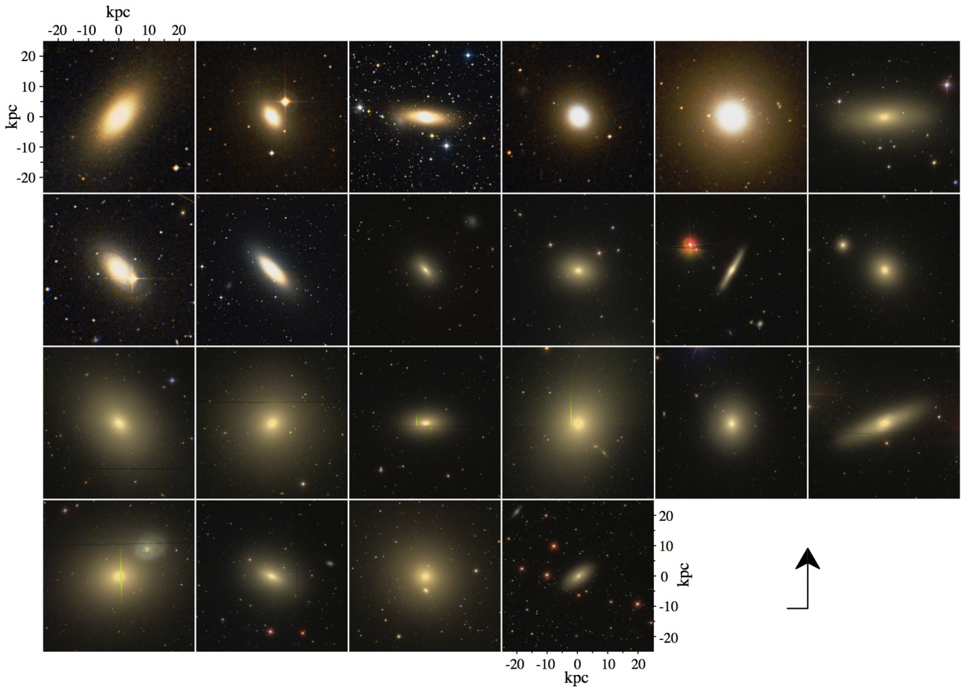
FIG. 2.— Color images of each galaxy, displayed on the same physical scale. The scale is indicated top left and lower right. Images were taken from the Sloan Digital Sky Survey (SDSS) where available, and the Digital Sky Survey (DSS) otherwise using sky-map.org. Galaxies are ordered left to right, top to bottom by ascending NGC number. Row 1: NGC 720, 821, 1023, 1400, 1407, 2768. Row 2: NGC 2974, 3115, 3377, 3608, 4111, 4278. Row 3: NGC 4365, 4374, 4473, 4486, 4494, 4526. Row 4: NGC 4649, 4697, 5846, 7457. The arrow indicates North up and East left.
