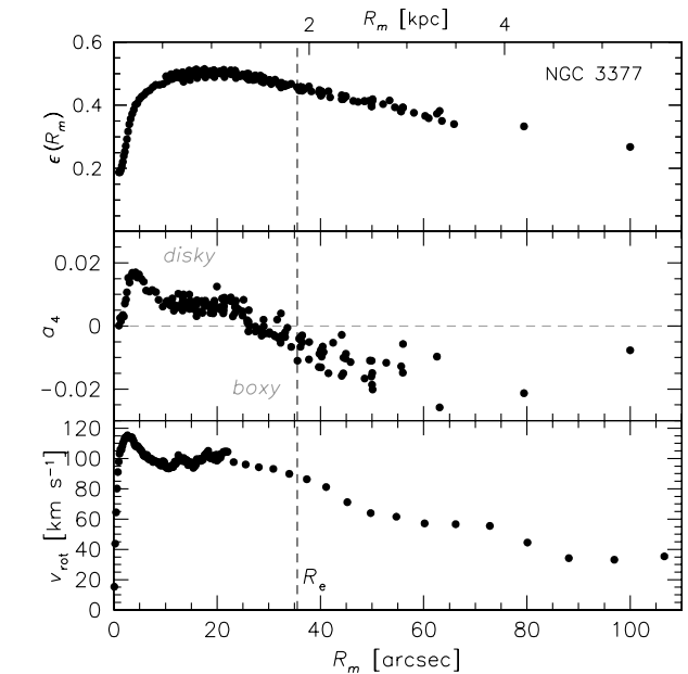
FIG. 13.— Two-dimensional photometry of NGC 3377. Left : g -band Subaru/Suprime-Cam image ( \sim 30 kpc field of view), with an arbitrary color scale used for contrast. Right : The top two panels show profiles of the isophote ellipticity and shape parameter (fourth-order cosine term a_4 > 0 is disk, < 0 is boxy, taken from literature studies in various optical filters; Jedrzejewski 1987; Michard & Simien 1988; Scorza & Bender 1995; Peletier et al. 1990; Goudfrooij et al. 1994). Both expressions of the data suggest a disk component embedded in a round and boxy bulge, which may be compared to the 1D rotation profile (bottom right panel) and to the 2D velocity map in Figure A1.
