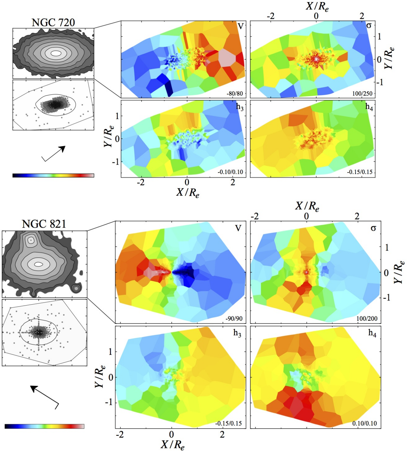
FIG. A1.— Smoothed kinematic maps of 22 early-type galaxies. A separate subplot for each galaxy includes a DSS image (top-left), a plot of stellar spectra (SLUGGS and literature) measurement locations (middle-left), and an arrow indicating North and East. In the data location plot the 1 R_e isophote is represented by a solid black ellipse, while each separate spectrum is denoted by a black dot surrounded by the convex hull of measurement locations (solid black polygon). Kinematic maps of V (center-top), \sigma (right-top), h_3 (center-bottom), and h_4 (right-bottom) are smoothed using the algorithm described in Section 4.1. The coloring scheme is set according to the colorbar (bottom-left), with the minimum/maximum of each range printed in the bottom right corner of each panel; V and \sigma are in \text{km s}^{-1} , h_3 and h_4 are unit-less. The color range is optimised for each galaxy. The plotted spatial scale, which varies from galaxy to galaxy, is only displayed for the \sigma and h_3 maps; with X - and Y -axes normalized by the R_e values listed in Table 1.
