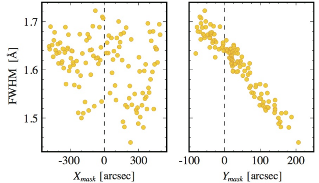
FIG. 5.— Spatial dependence of DEIMOS spectral resolution. Left Measured resolution as a function of x -position and Right y -position across a single DEIMOS slit mask. FWHM values are measured from a night sky emission line (at 8415 \text{\AA} ) in the background spectrum of each slit. The resolution appears uncorrelated with x -position on the mask (long axis), but has a dependence on y -position (short axis).
