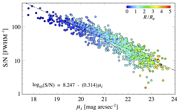
FIG. 4.— Photometric depth of the DEIMOS measurements. Spectral S/N is plotted versus the local i -band surface brightness around each measurement location. Surface brightness values are measured from SDSS images, and only spectra from those galaxies within the SDSS footprint are shown. Points are colored according to galactocentric radius normalized by R_e (see color bar at top-right). There is a roughly linear relation, shown as a dot-dash line and given at bottom left, between the base-10 logarithm of the spectral S/N and the local surface brightness.
