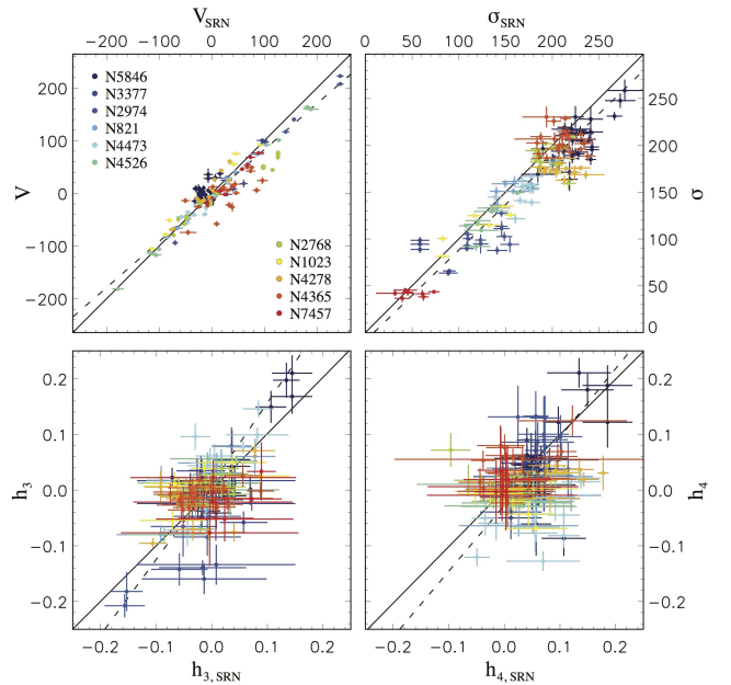
FIG. 8.— Literature comparison of kinematic measurements. Comparison between our measured values (y axes) and literature values from the SAURON (SRN) survey (x axes). Velocity (top left), velocity dispersion (top right), h_3 (bottom left), and h_4 (bottom right). Points are color coded according to galaxy, as shown in the key in the top-left panel. The solid black line is a 1:1 relation, while the dot-dashed line denotes the best fitting linear relation to the data that takes the x and y error bars into consideration. See text for details.
