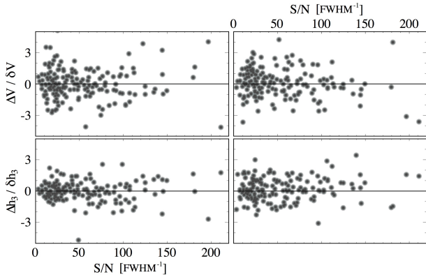
FIG. 7.— Repeatability of measured velocity moments. The difference ( \Delta ) between measurements from spectra that are co-spatial to within 3 arcseconds versus S/N per resolution element. Each \Delta value is normalized by the measurement errors added in quadrature. If the derived errors, for Velocity (top left), velocity dispersion (top right), h_3 (bottom left), and h_4 (bottom right), fully accounted for the true measurement error, then the standard deviation of the values on the y-axis would be exactly 1 in each panel. However, at high S/N, both velocity and velocity dispersion show anomalously high values, suggestive of underestimated errors or a small systematic error term (see text).
