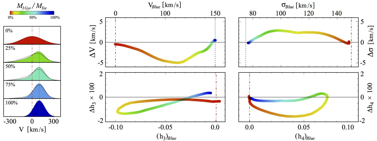
FIG. C1.— Differential kinematic effects of a young stellar component on blue and red spectral regions. Composite spectra of single stellar populations are created by combining spectra together from a 3 Gyr and a 10 Gyr old population. The input spectra are first convolved with Gaussian LOSVDs (i.e. V = 100 \text{ km s}^{-1} and \sigma = 75 \text{ km s}^{-1} ). Fiducial composite LOSVDs are shown (left) and colored according to young star fraction. Each panel (middle and right) shows the difference between the measured LOSVD parameters for red spectra centered on the calcium triplet (8480–8750 Å) and blue spectra (4800–5380 Å). If both spectral regions were equally sensitive to young stars, the curves would all be horizontal indicating exactly equal measurements. While there is some obvious differential sensitivity apparent, the amplitude of the difference is small enough to be ignored, given the typical uncertainties on these parameters for our spectra.
