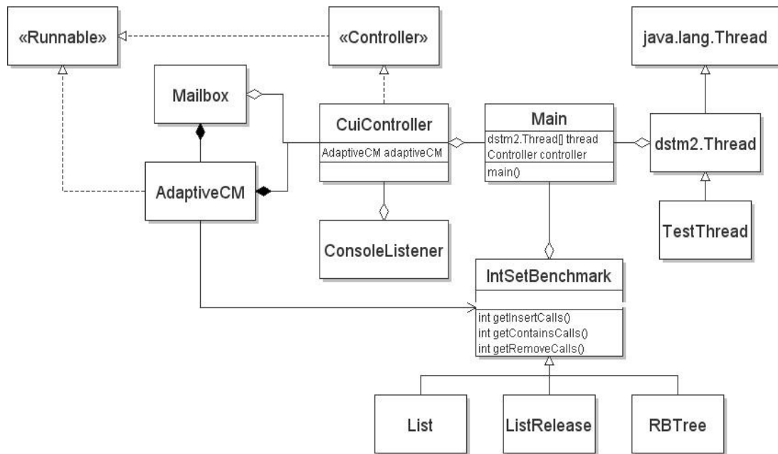
Figure 5 - Overview UML
