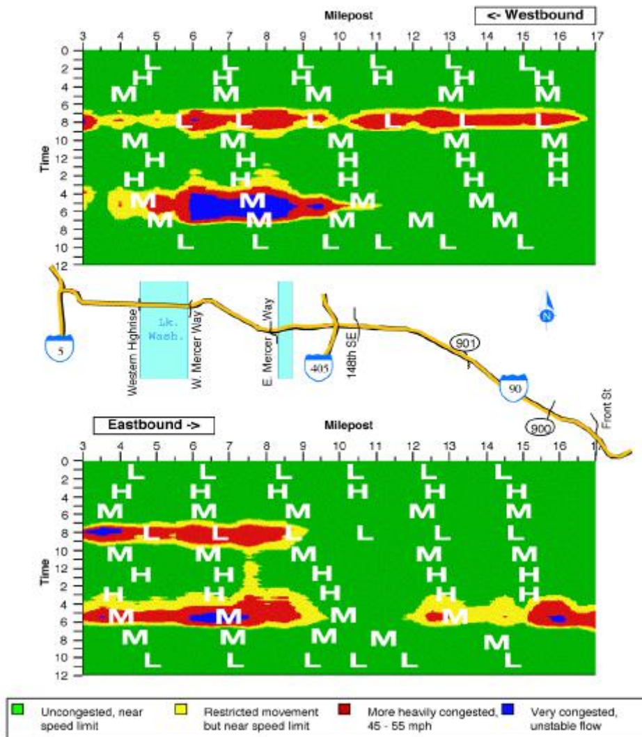
Figure 10: Illustration of Method for Displaying Relative Truck Volume on Space-Time Plot of Freeway Traffic Congestion
