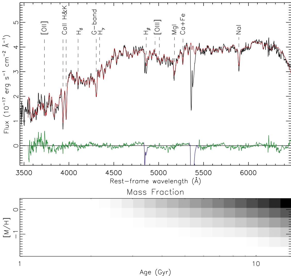
Figure 2. (Upper panel) Relative flux calibrated Gemini spectrum (black) of the host galaxy of XJ1417+52 vs. the source rest-frame wavelength, with the best-fitting pPXF model (red) and residuals (green/blue) overplotted. The two drops at around 4844 Å and 5360 Å (corresponding to 6870 Å and 7604 Å, respectively, in the observer frame; indicated by the blue residuals), are due to the atmospheric OH absorption and were excluded in the fit. The spectrum bluer than 3541 Å was not fitted because the stellar models do not cover this wavelength range. Important stellar absorption and AGN diagnostic emission lines are denoted for reference. For clarity, we have smoothed data points with a boxcar function with width 5 pixels for clarity. (Lower panel) Relative mass fractions of different stellar populations with respect to metallicity and age, with darker shading indicating a larger mass fraction in the best-fitting model.
