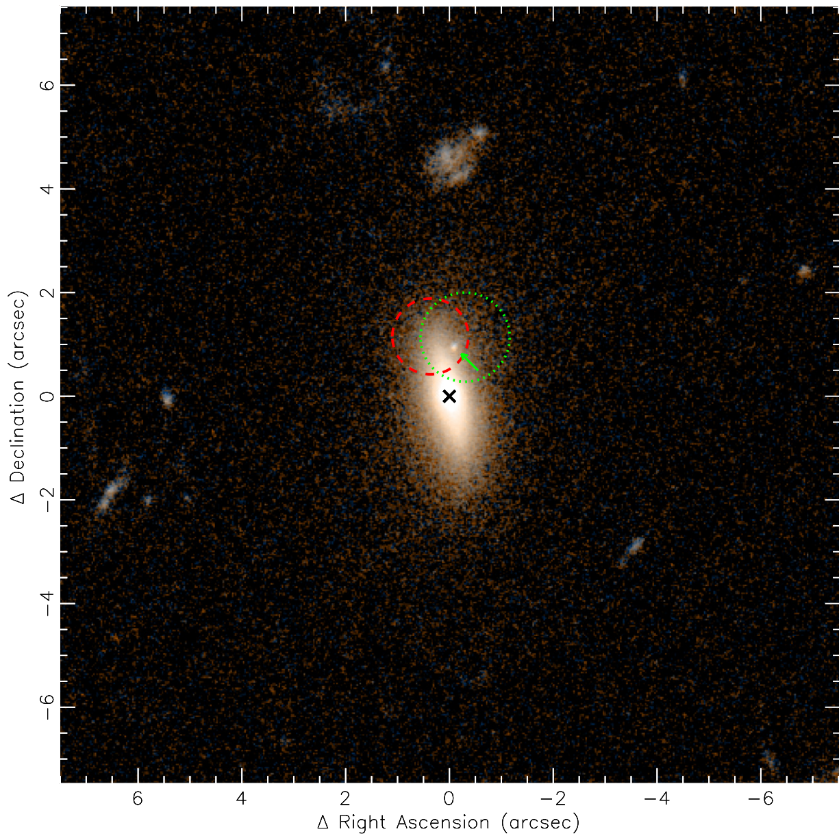
Figure 1. HST /ACS/WFC multidrizzled image in the field of XJ1417+52, with the origin at the center of the galaxy GJ1417+52 (black cross, R.A. = 14:17:11.076, Decl.=+52:25:40.80). The angular scale of GJ1417+52 is 5.5 kpc/1". The image is false-colored, using the F814W (red) and F608W (blue) images and their mean (green). The green arrow points to a faint optical source sGJ1417+52 at R.A. = 14:17:11.066 and Decl.=+52:25:41.74. The 95% positional error (0".73) of XJ1417+52 from the XMM-Newton observations is marked as a red dashed circle, and that (0".86) from the Chandra observations as a green dotted circle, both indicating that the faint optical source could be the counterpart to our X-ray source.
