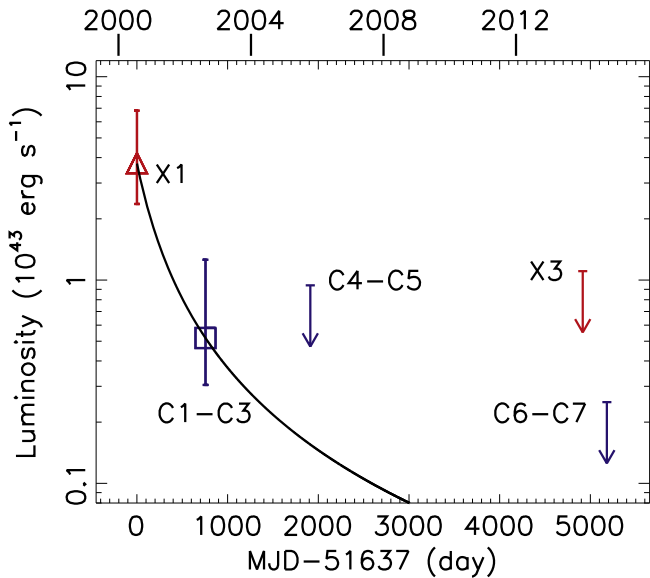
Figure 4. The long-term rest-frame 0.28–14.2 keV unabsorbed luminosity curve, with 90% uncertainties or 3\sigma upper limits (see Table 1). For clarity, X2 is not plotted because it is only two days after X1 and had a similar luminosity (but with a larger uncertainty). The solid line represents a (t - t_D)^{-5/3} decline passing through the X1 and C1–C3 data points, which implies the disruption time t_D to be \sim 11 months before X1.
