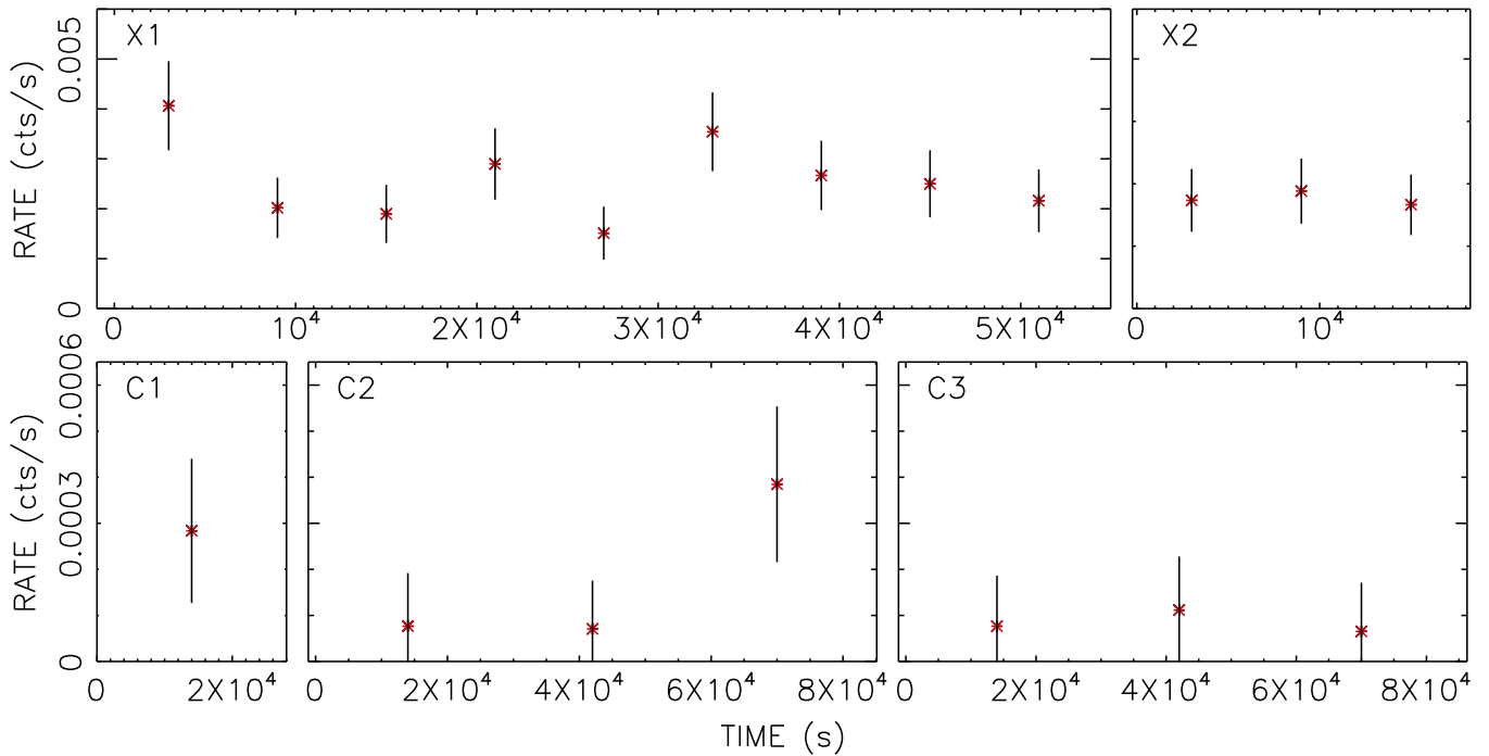
Figure 5. The background subtracted light curves for XMM-Newton observations X1 and X2 (upper panels, MOS1 camera, 0.2–1 keV, bin size 6 ks) and for Chandra observations C1–C3 (lower panels, 0.3–1 keV, bin size 28 ks). We note that X1 and X2 are separated by two days, while C2 is one day after C1 and C3 is nine days after C2. The 1\sigma uncertainties are included, and they are calculated following Gehrels (1986) for the Chandra observations due to low counts of most data points.
