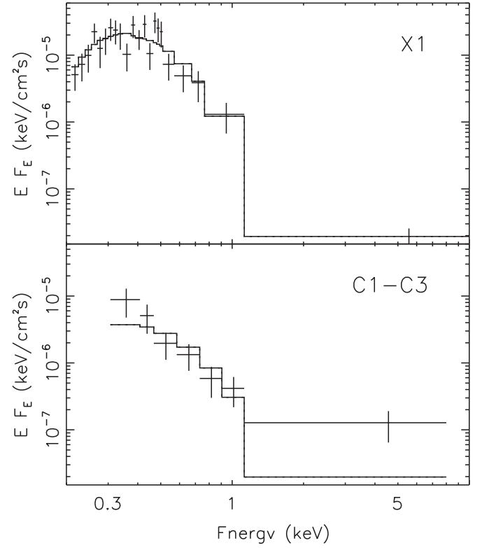
Figure 3. The unfolded spectra of X1 (upper panel, for clarity, only the MOS1 spectrum is shown) and C1–C3 (lower panel) from the MCD fits. For clarity, the spectra were rebinned to be above 2\sigma per bin in the plot.
