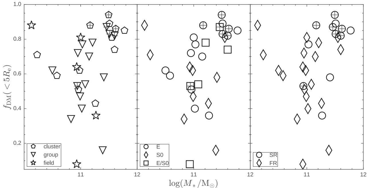
Figure 5. DM fraction versus total stellar mass, highlighting different galaxy environments in the left-hand panel, galaxy morphologies in the middle panel and galaxy central kinematics in the right-hand panel (SR = slow rotators; FR = fast rotators). Centrally dominant galaxies have been marked with black crosses and they mostly have high DM fractions. As a function of morphology, DM fraction appears to increase with galaxy stellar mass in ellipticals while lenticulars show a noisy, somewhat decreasing trend with mass and a lower median f_{\text{DM}} compared to elliptical galaxies. The decreasing trend with stellar mass in lenticulars from the middle panel is not seen in the fast rotators in the right-hand panel.
