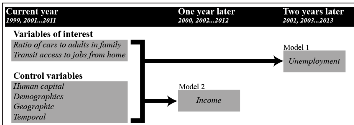
Figure 10. Modeling Approach
