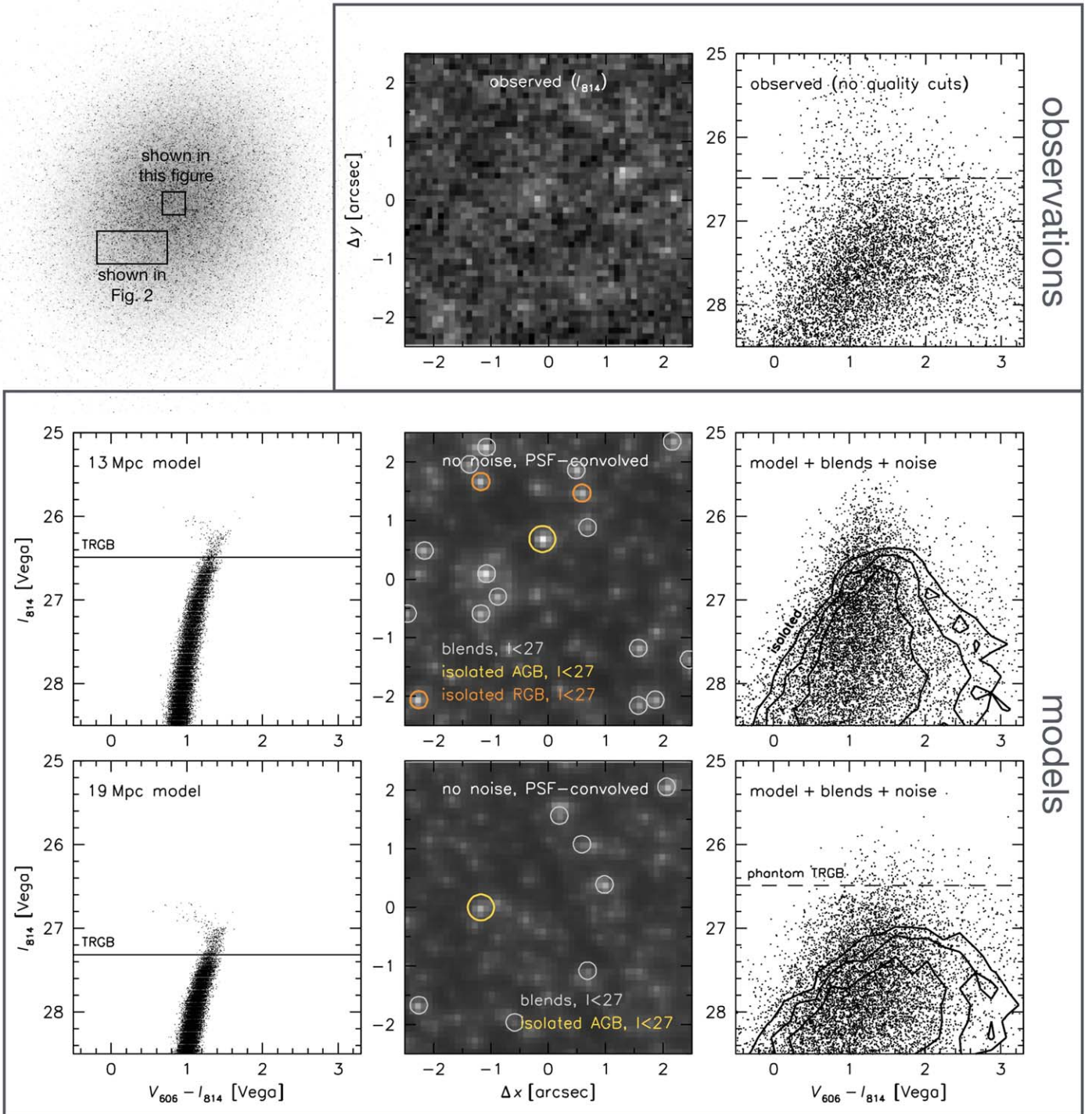
Figure 1. Comparison of the CMD of NGC 1052–DF2 (top right; prior to applying quality cuts to eliminate blends) to models at distances of 13 Mpc (middle row) and 19 Mpc (bottom row). The models reproduce the global properties of NGC 1052–DF2. The observed “raw” CMD shows a ridge line at I_{814} \approx 26.5 . The images in the middle column show the central 5'' \times 5'' of the data and the models. Circles indicate detectable isolated stars and blends; most of the brightest compact objects are blends. The distributions of isolated stars in the CMDs are indicated with contours in the panels on the right. Taking blends and photometric errors into account the model CMD for 19 Mpc is a good match to the data, including the “phantom” TRGB at I_{814} \approx 26.5 .
