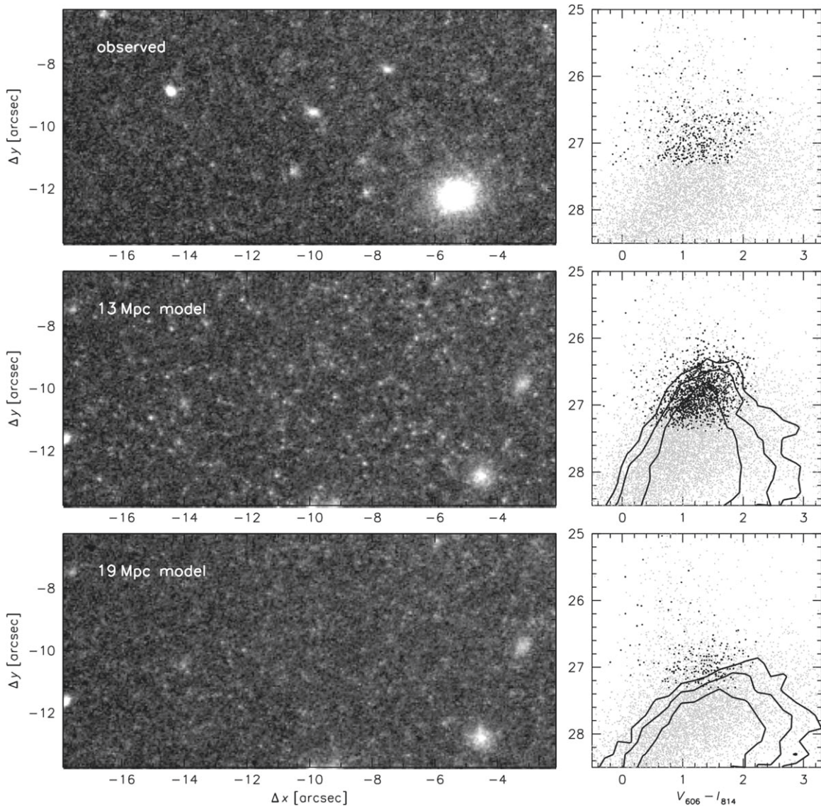
Figure 2. Comparison of NGC 1052–DF2 to artificial galaxy images placed in the HST /ACS data (see Figure 1 for their location). The CMDs measured with DOLPHOT are shown on the right. Gray points are “raw” photometry; black points are objects that survive standard quality cuts. Contours are repeated from Figure 1 and show the expected distribution of isolated stars. For a distance of 13 Mpc the HST images would have shown a large number of isolated stars above the detection limit.
