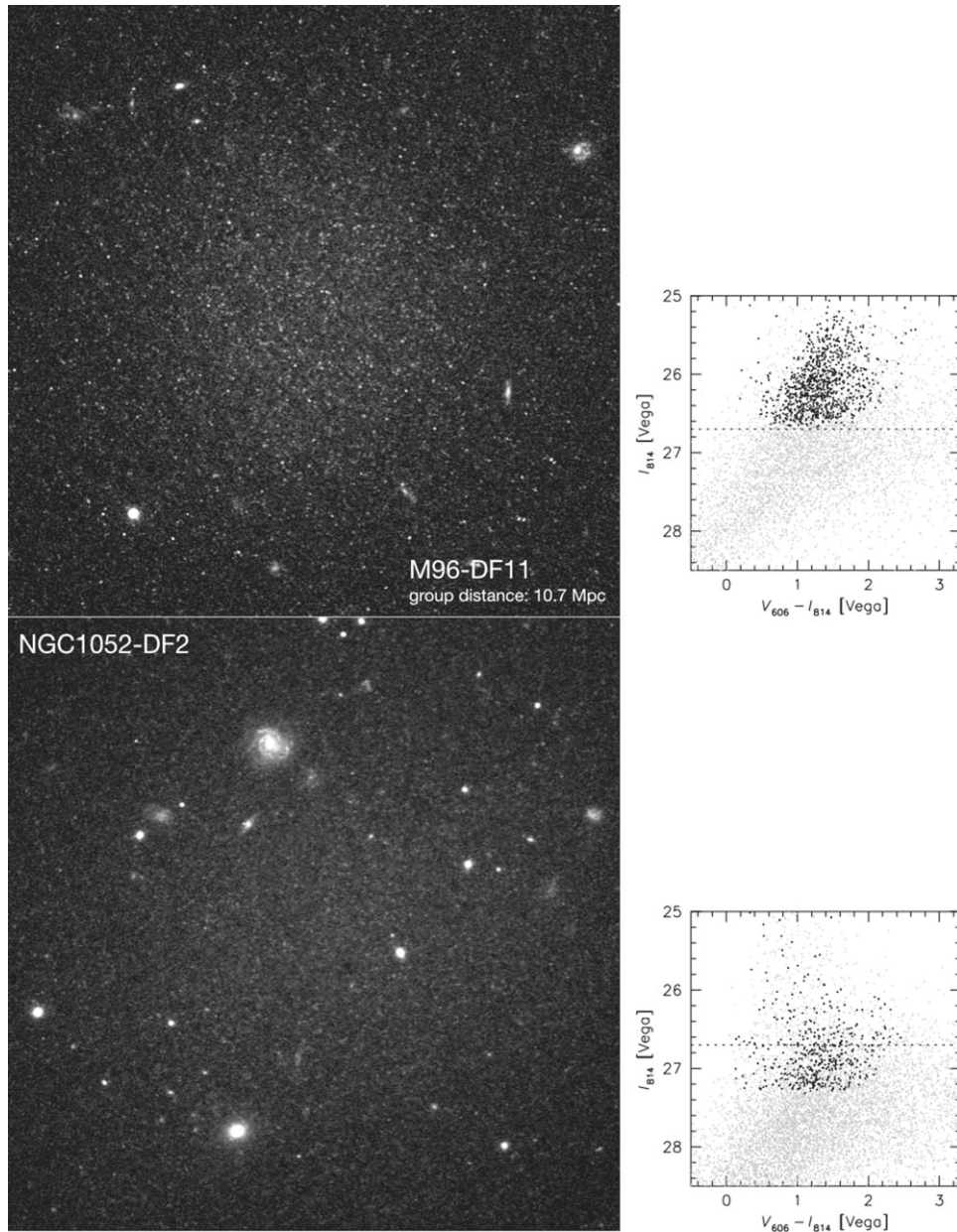
Figure 3. NGC 1052–DF2 and M96–DF11 (C18) have very similar surface brightness, size, morphology, and integrated color. The images span 21'' \times 21'' . Gray dots in the CMD are all detections; black dots are what remains after quality cuts. The broken line indicates the depth of the (half-orbit) M96–DF11 I_{814} data. For M96–DF11 we reach below the tip of the giant branch, and the galaxy takes on a resolved appearance. The distance to the M96 group is 10.7 \pm 0.3 Mpc (see Section 4). The distance to NGC 1052–DF2 is clearly much greater.
