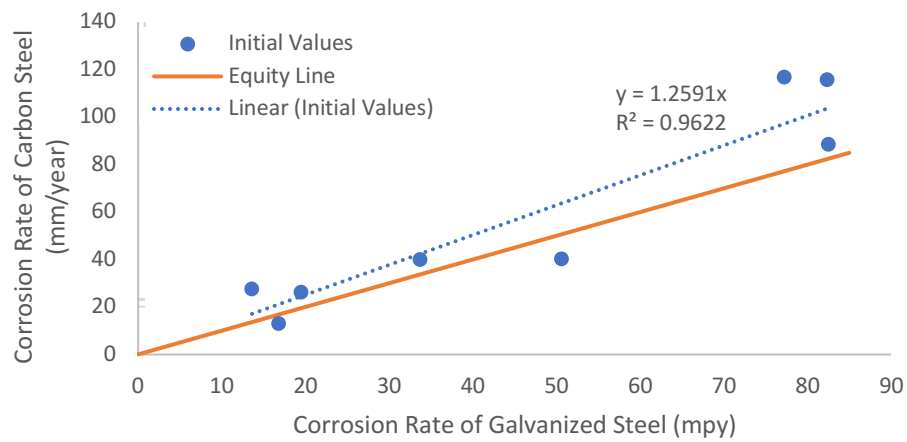
Figure 64. Comparing Corrosion Rates of Galvanized and Carbon Steel Coupons
