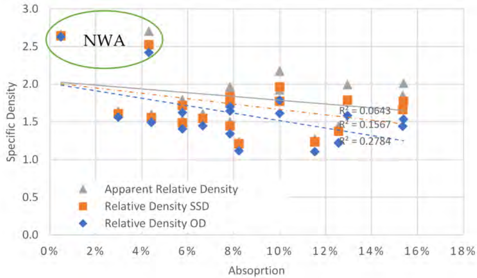
Figure 29. Density-absorption Trends of Sample Aggregates
