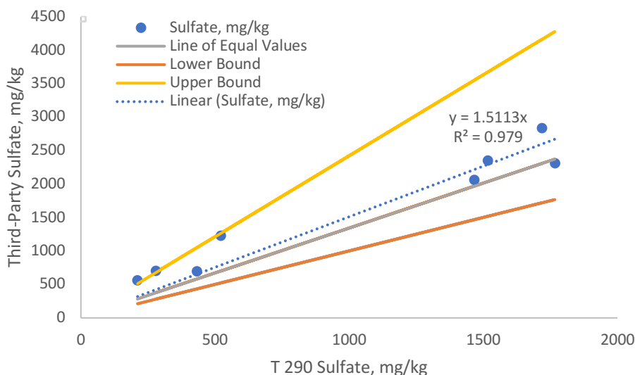
Figure 52. Verification of Sulfate Results with the Third-Party Laboratory Results
