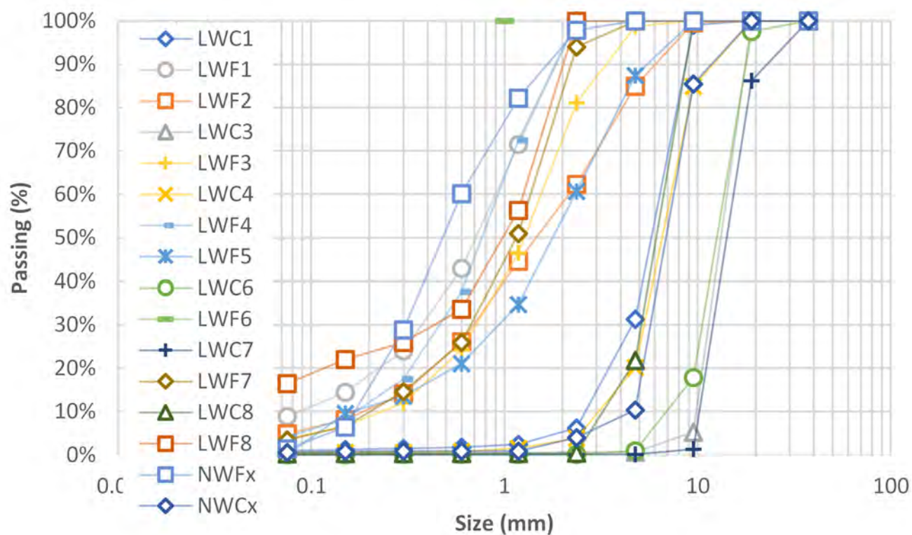
Figure 27. Sieve Analysis of Sample Aggregates
