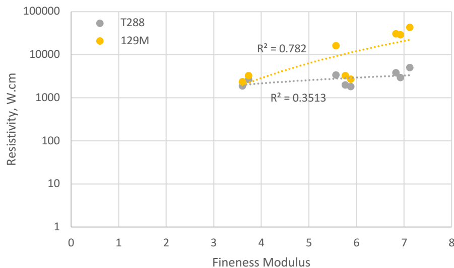
Figure 42. Electrical Resistivity as a Function of Fineness Modulus
