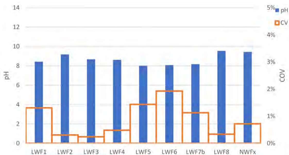
Figure 43. pH of Selected Samples Using AASHTO T 289
