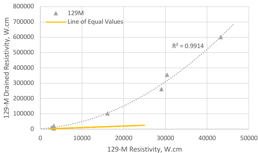
Figure 40. Comparing Electrical Resistivity of Saturated and Drained Conditions
