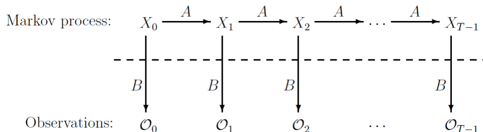
Figure 10. Hidden Markov Model [1]
