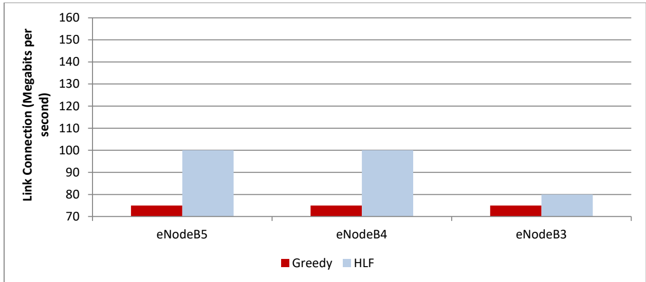
Figure 22: Link Connection for Architecture2 in a Non-Uniform Data traffic
