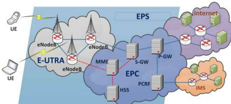
Figure 3: Telecommunications Architecture [6]
