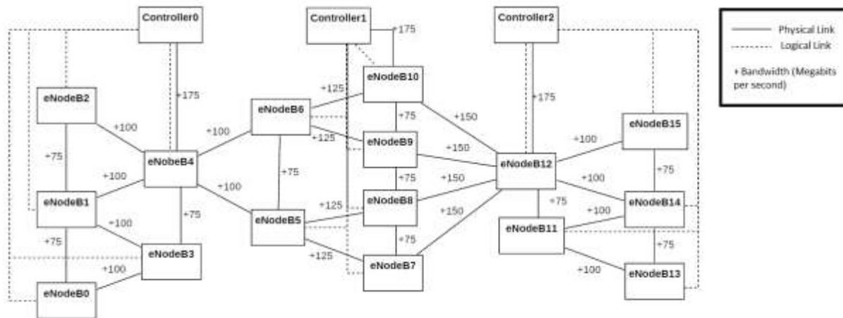
Figure 9: Failover Architecture1
