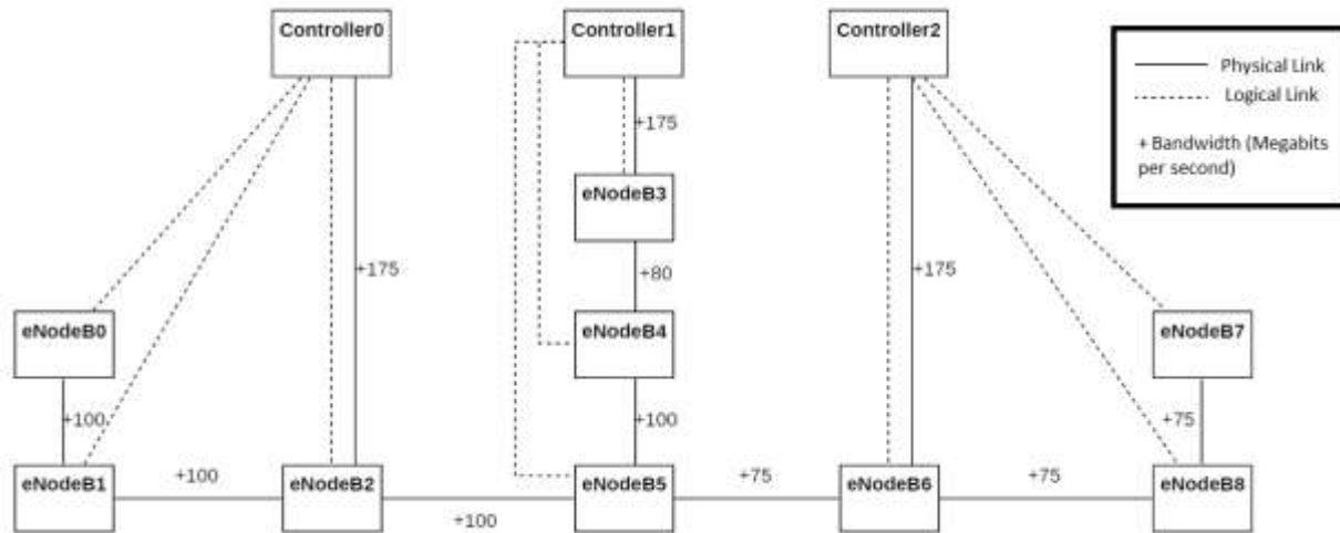
Figure 10: Failover Architecture2
