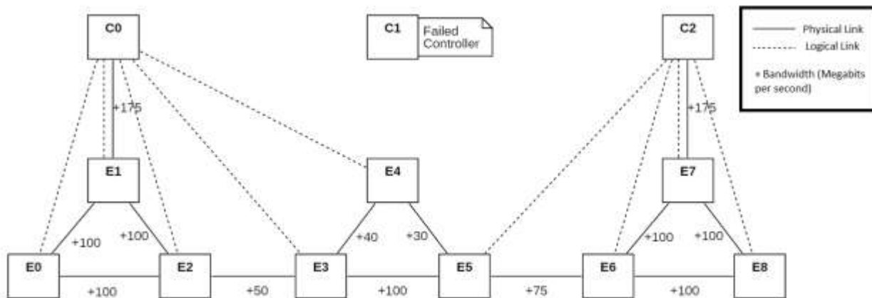
Figure 8: Final Architecture
