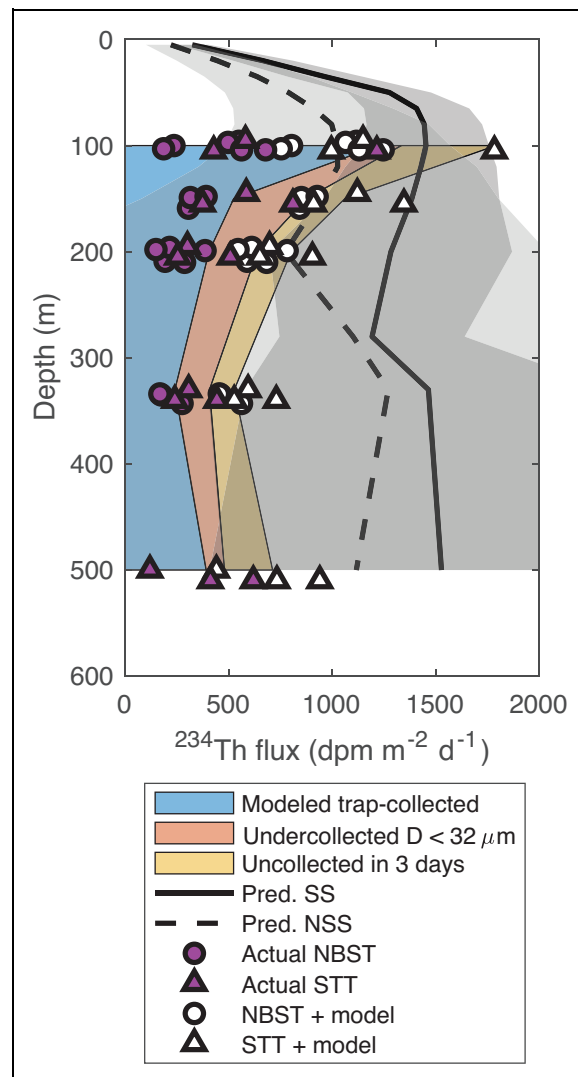
Figure 11. Measured, modeled, and predicted contributions to 234 Th flux averaged during the cruise. Filled colored areas illustrate the cumulative contributions to the 234 Th flux modeled from extrapolated sinking particle size distributions (see text). These include modeled flux of particles of diameter ( D ) larger than 32 μm collected by traps (blue, “Modeled trap-collected”), flux carried by smaller, potentially undercollected particles (orange), and flux carried by rare, infrequently collected particles (yellow). Also shown are the predicted 234 Th flux from the steady-state (SS) model that assumes flux is constant in time (solid black line and shaded dark gray area showing uncertainty; see text discussion and Buesseler et al., 2020a) and from the non-steady-state (NSS) model that allows for time-varying flux (dashed black line and shaded light gray area; see text discussion and Buesseler et al., 2020a), as well as the measured flux in the neutrally buoyant sediment traps (NBSTs; magenta circles) and surface-tethered traps (STTs; magenta triangles), and the same trap fluxes with added, modeled contributions by small and infrequently collected particles (white symbols). DOI: https://doi.org/10.1525/elementa.2020.00122.f11
