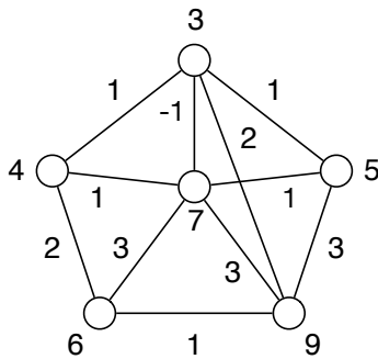
Figure 8: IAM(W_5^+) = \{7, 8, 9, \dots\} .
