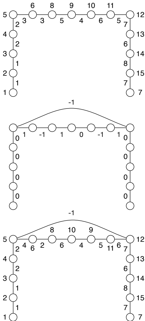
Figure 4: IAM(P_{15}(6)) = \{15, 16, 17, \dots\} .
