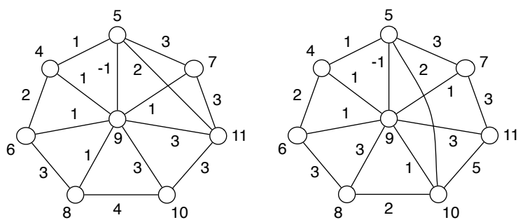
Figure 10: IAM(W_7^+) = \{8, 9, 10, \dots\} .
