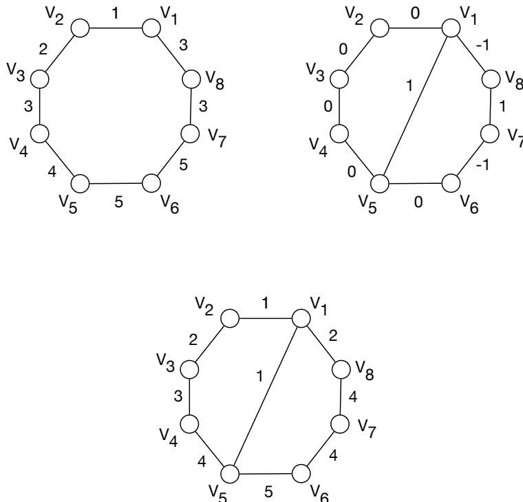
Figure 3: IAM(C_8(4)) = \{8, 9, 10, \dots\} .
