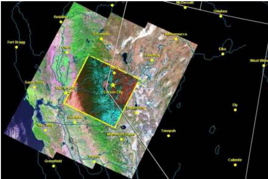
Figure 1- Landsat image of Path 43 Row 33, outlined in yellow, in relation to cities in California and Nevada. Image generated using the USGS Global Visualization Viewer.
